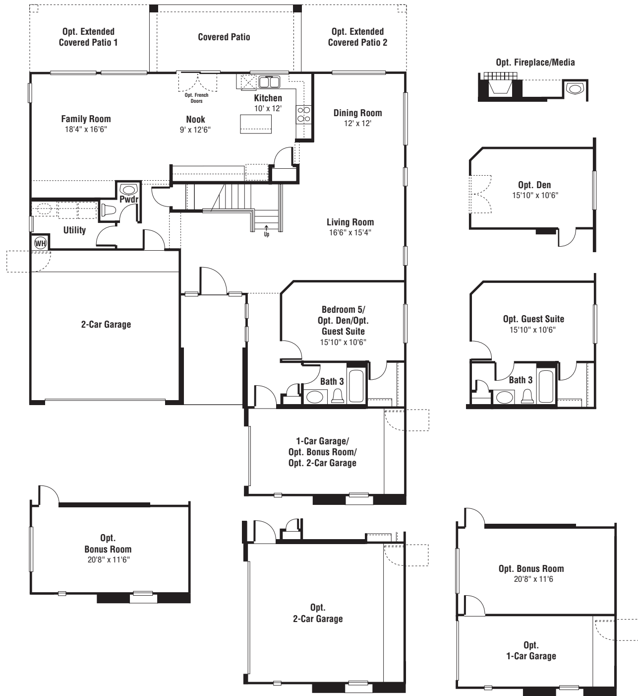
First Floor
