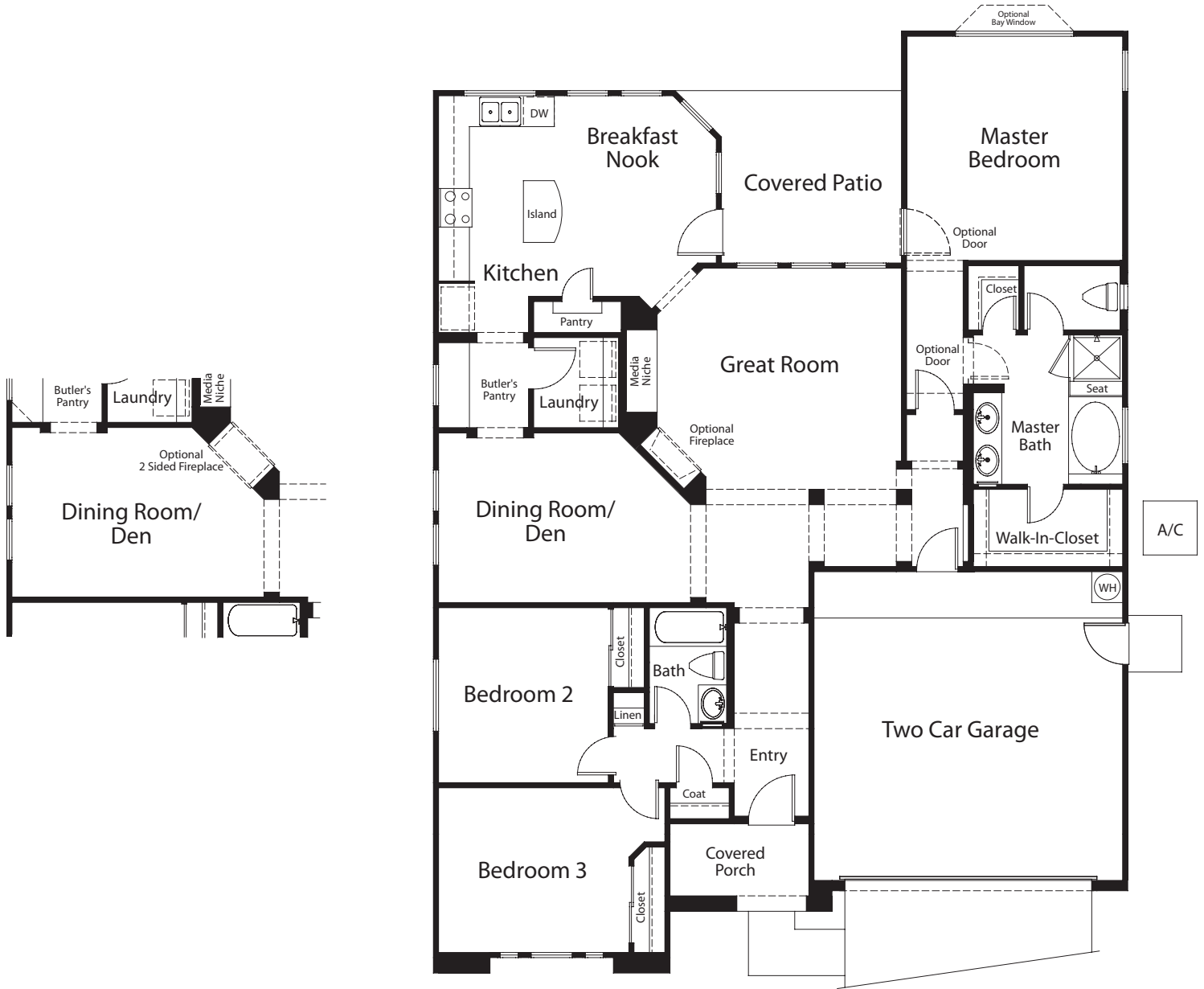
Floor plan shown is "A" elevation
